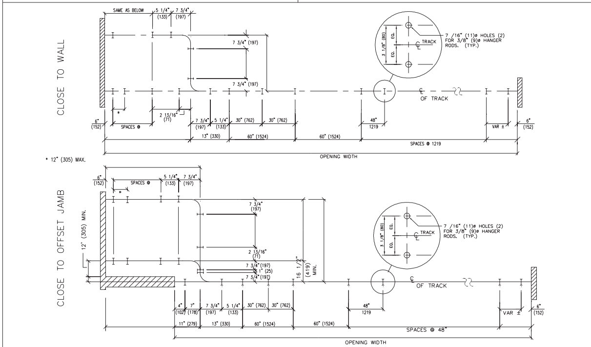
PUNCHING TEMPLATE
