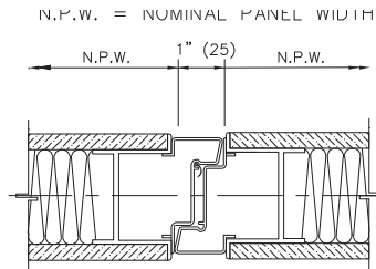
(C) CLOSURE DETAIL
